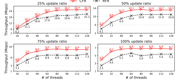
Figure 12: Performance comparison of RNIC-friendly RPC and coroutine-friendly RPC (§IV-D). We use uniform distribution to minimize the effects of contention. Each thread is configured with two coroutines.
